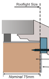
Figure 5: rooflight with builders upstand detail
