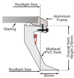
Figure 6: rooflight with 150mm PVC kerb detail
