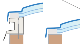
Structural, Insulated Builders upstand - Direct Fix kerb supplied for vented and opening variants
