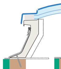
Standard 150mm PVCu* - kerb type varies with specification
