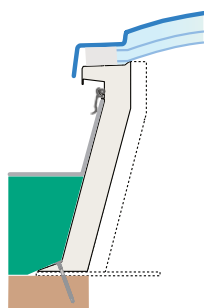
Tall 300mm PVCu*
